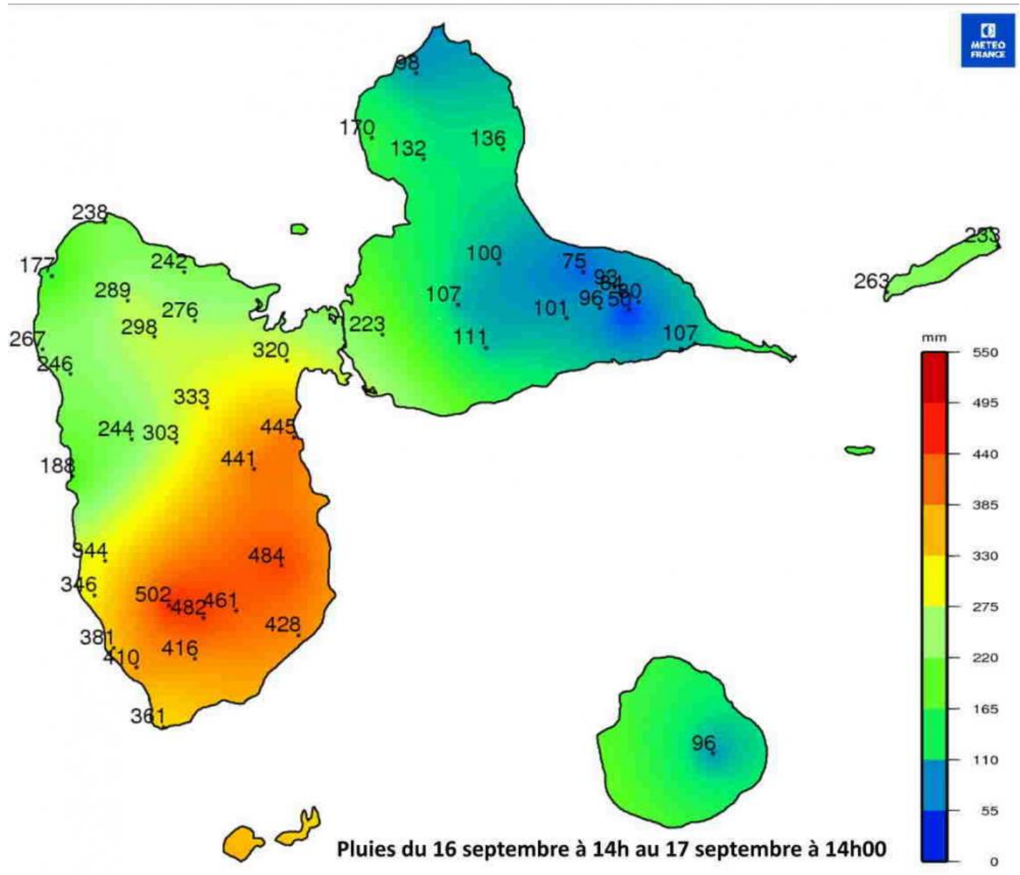
Figure 5. Rainfall accumulations (mm) from Fiona in Guadeloupe. Image courtesy of Météo France.
