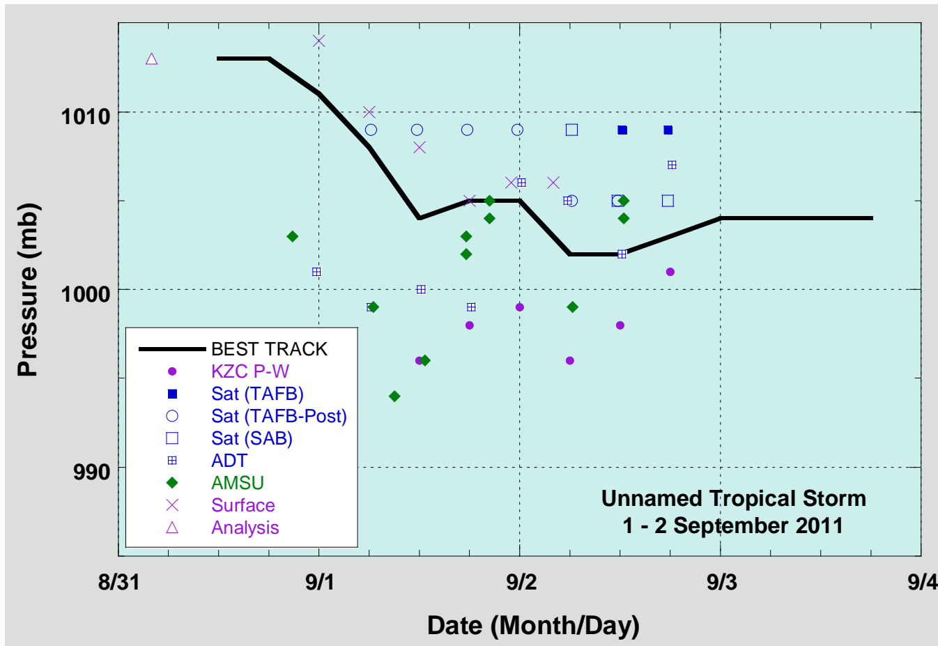
Figure 3. Selected pressure observations and best track minimum central pressure curve for the Unnamed Tropical Storm, 1 – 2 September 2011. Advanced Dvorak Technique estimates represent linear averages over a 3-hr period centered on the nominal observation time. AMSU intensity estimates are from the Cooperative Institute for Meteorological Satellite Studies technique. The KZC P-W values are obtained by applying the Knaff-Zehr-Courtney pressure-wind relationship to the best track wind data. Estimates during the extratropical stage are based on analyses from the NOAA Ocean Prediction Center. Dashed vertical lines correspond to 0000 UTC.
