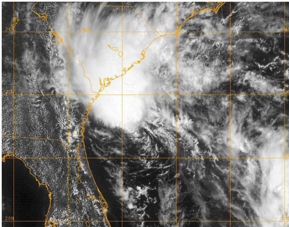
GOES-13 VISIBLE IMAGE OF BONNIE AT PEAK INTENSITY (1900 UTC 28 MAY 2016). IMAGE COURTESY OF THE U.S. NAVAL RESEARCH LABORATORY TC WEBPAGE.
