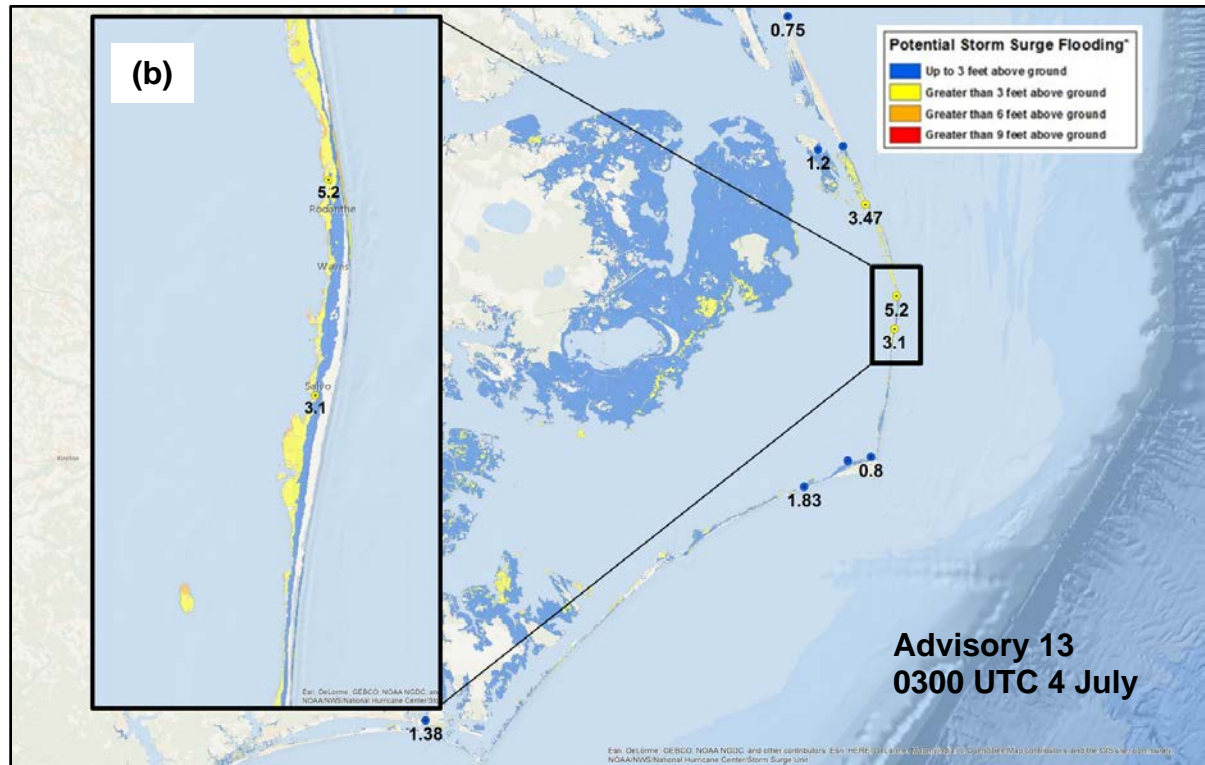
Figure 8. Measurements of storm surge inundation (in ft above ground level) verified against the experimental Potential Storm Surge Flooding Maps issued during Hurricane Arthur for (a) Advisory 7 (1500 UTC 2 July) and (b) Advisory 13 (0300 UTC 4 July). The inset on both figures provides a close-up view of the Rodanthe-Salvo area where the highest inundation occurred.
