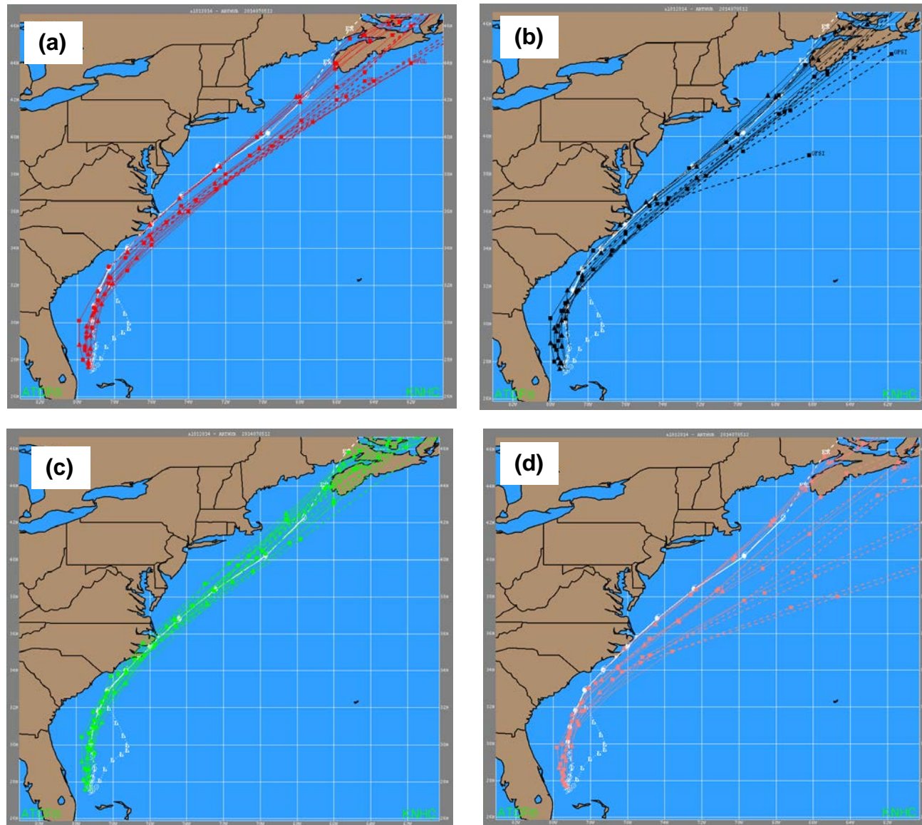
Figure 6. (a) Official track forecasts, (b) GFS forecasts, (c) HWRP forecasts, and (d) ECMWF forecasts for Hurricane Arthur, 1-5 July 2014 from 0000 UTC 1 July through 1200 UTC 5 July. The best track is given by the thick solid white line with positions given at 6-h intervals.
