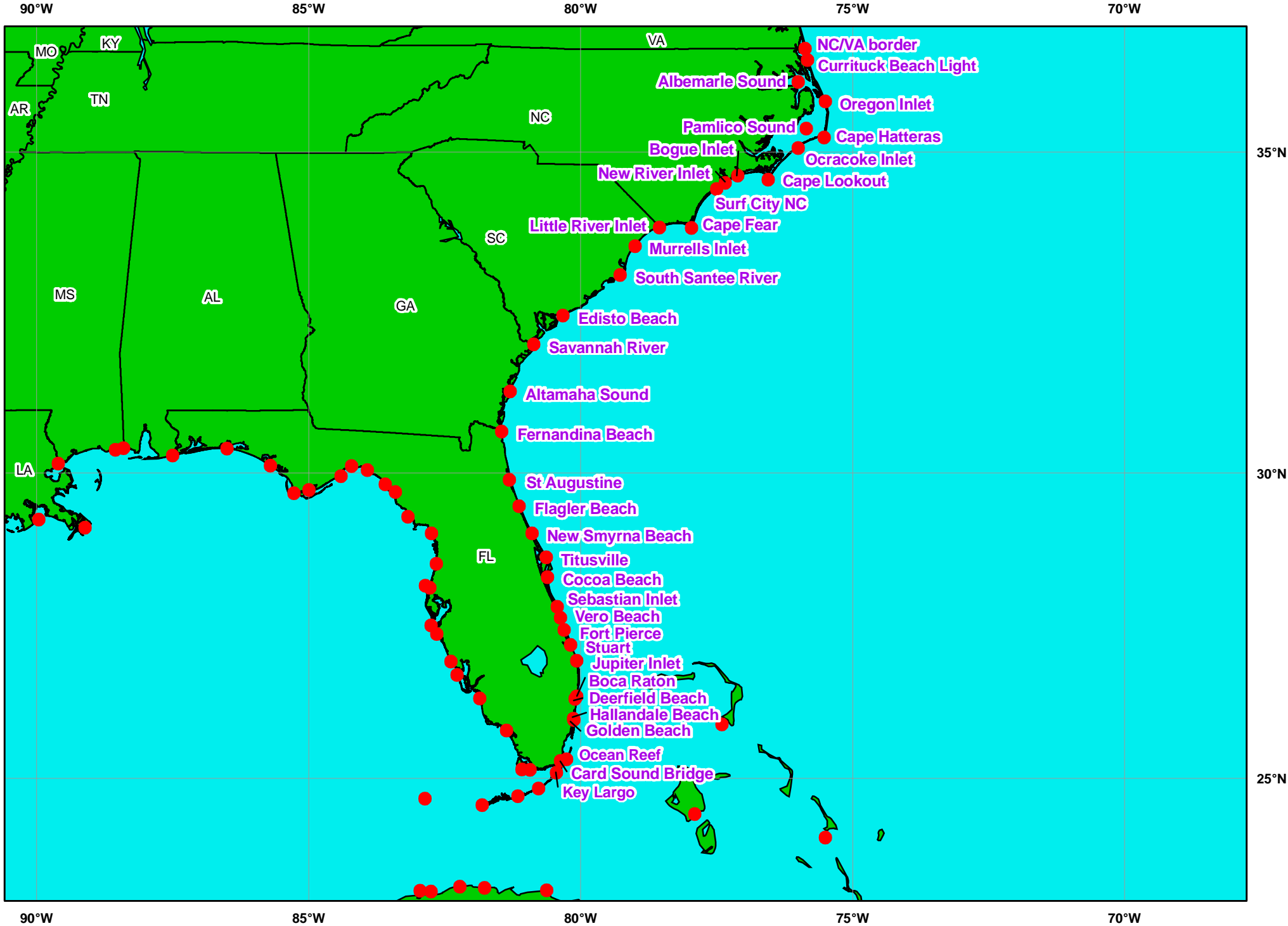
TROPICAL CYCLONE BREAKPOINTS - SOUTHEAST
