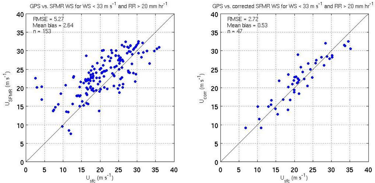
Fig. 3: Comparison of U_{SFMR} vs U_{sfc} for wind speeds < 33 m/s and R > 20 mm/hr (left), and comparison for U_{corr} vs. U_{sfc} for same range based on independent observation sample.
