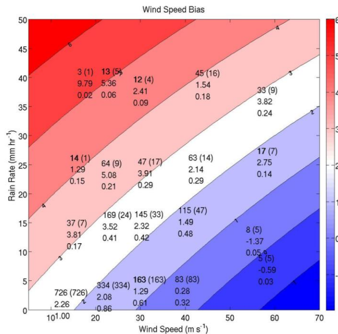
Fig. 2: Fitted wind speed bias ( \Delta U ) function computed from Eq. 2. Contours are every 1 \text{ m s}^{-1} with warmer colors representing higher biases and colder colors representing lower biases. Values are located at the mean wind speed and rain rate within each bin. The top line of each text field on the figure is the pair count with the number of real data in parentheses. The second line is the weighted mean difference for each bin, and the third line is the weight applied to the particular bin.
