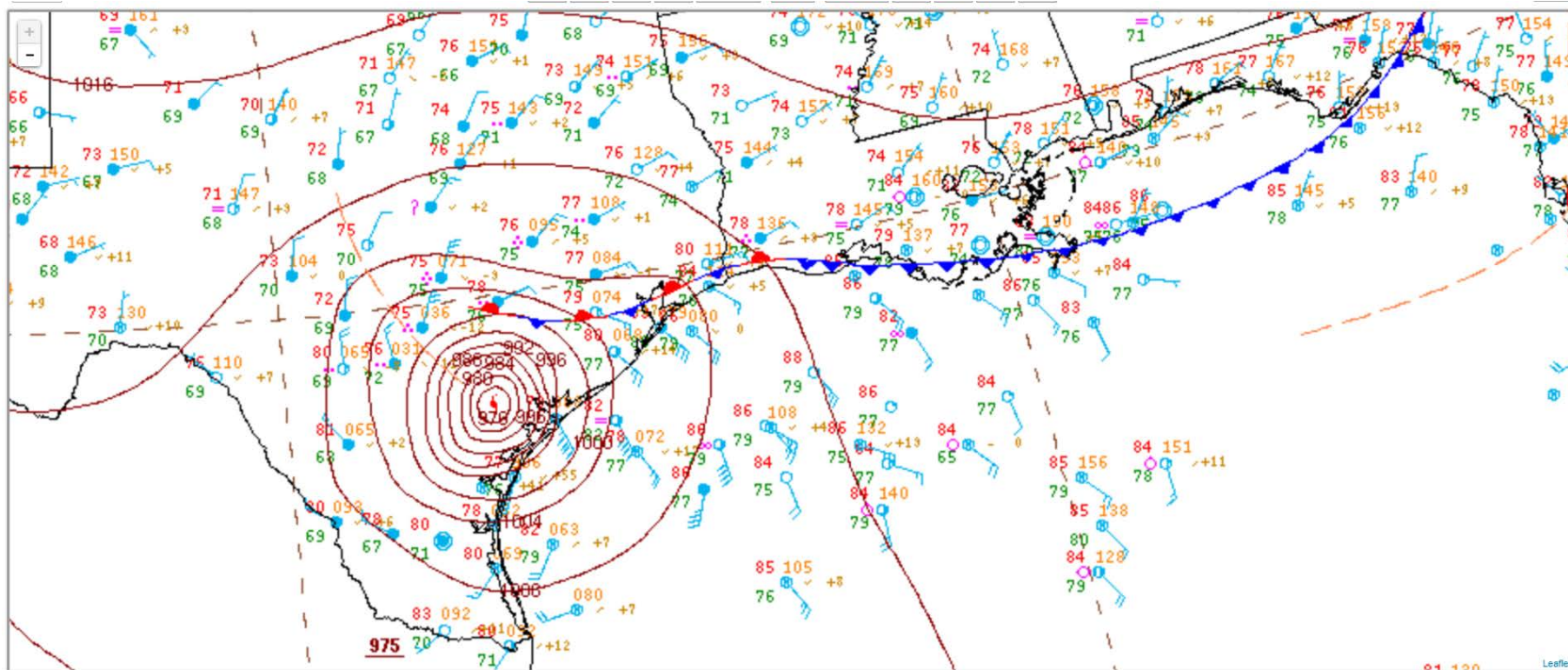
Figure 13. NCEP unified surface analysis at 1200 UTC 26 August 2017.
