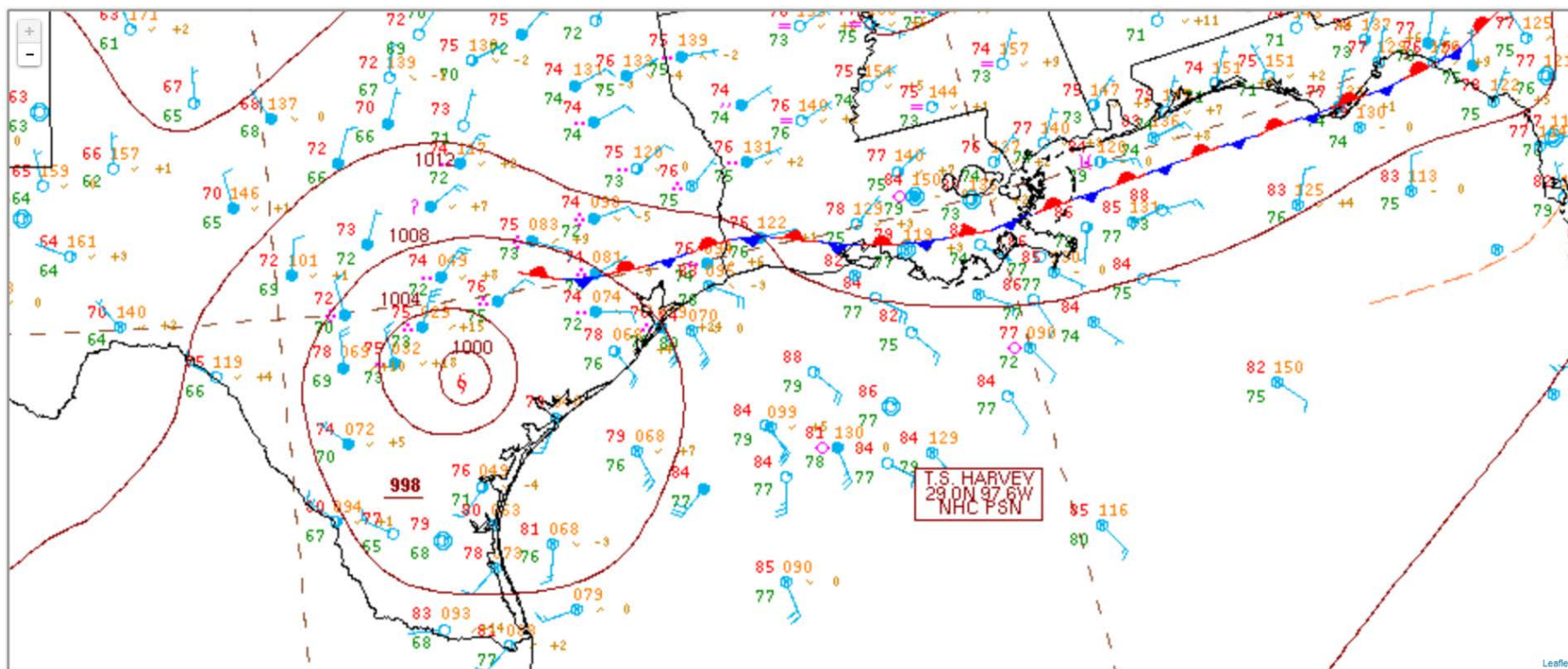
Figure 14. NCEP unified surface analysis at 1200 UTC 27 August 2017.
