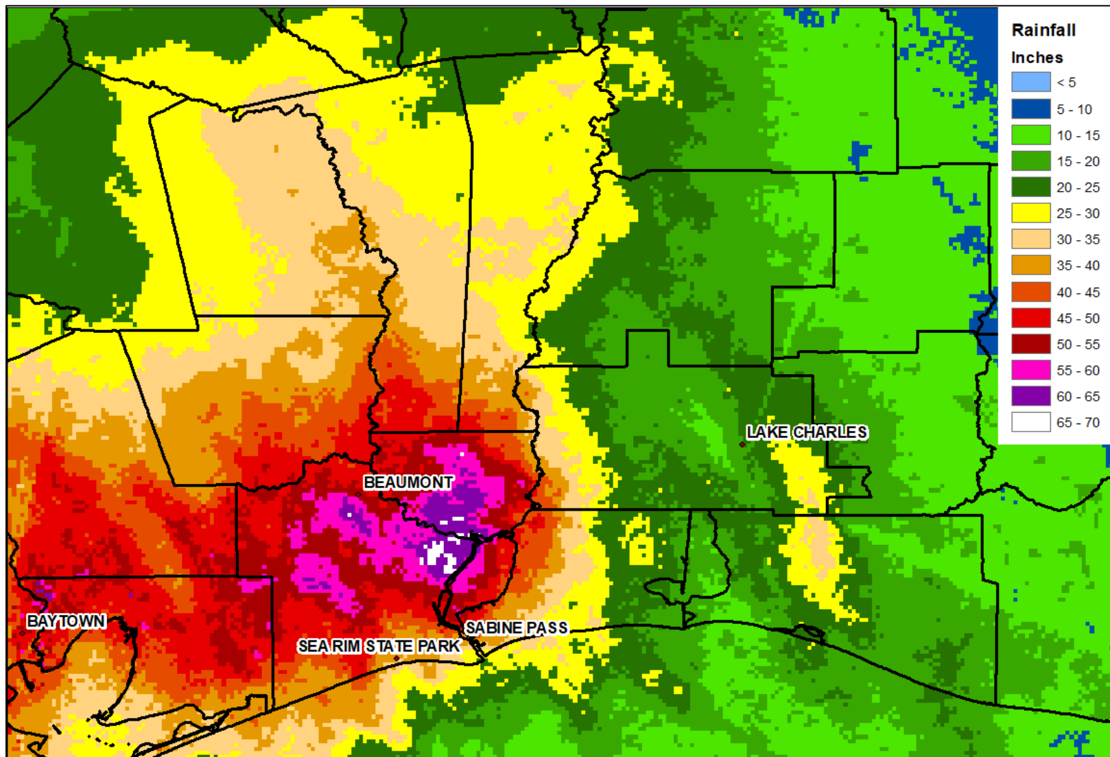
Figure 10. Raw NOAA Multi-radar multi-sensor quantitative precipitation estimation (inches) for Harvey in southeastern Texas from 25 August to 1 September 2017. Figure courtesy Jonathan Brazzell of NWS Lake Charles.
