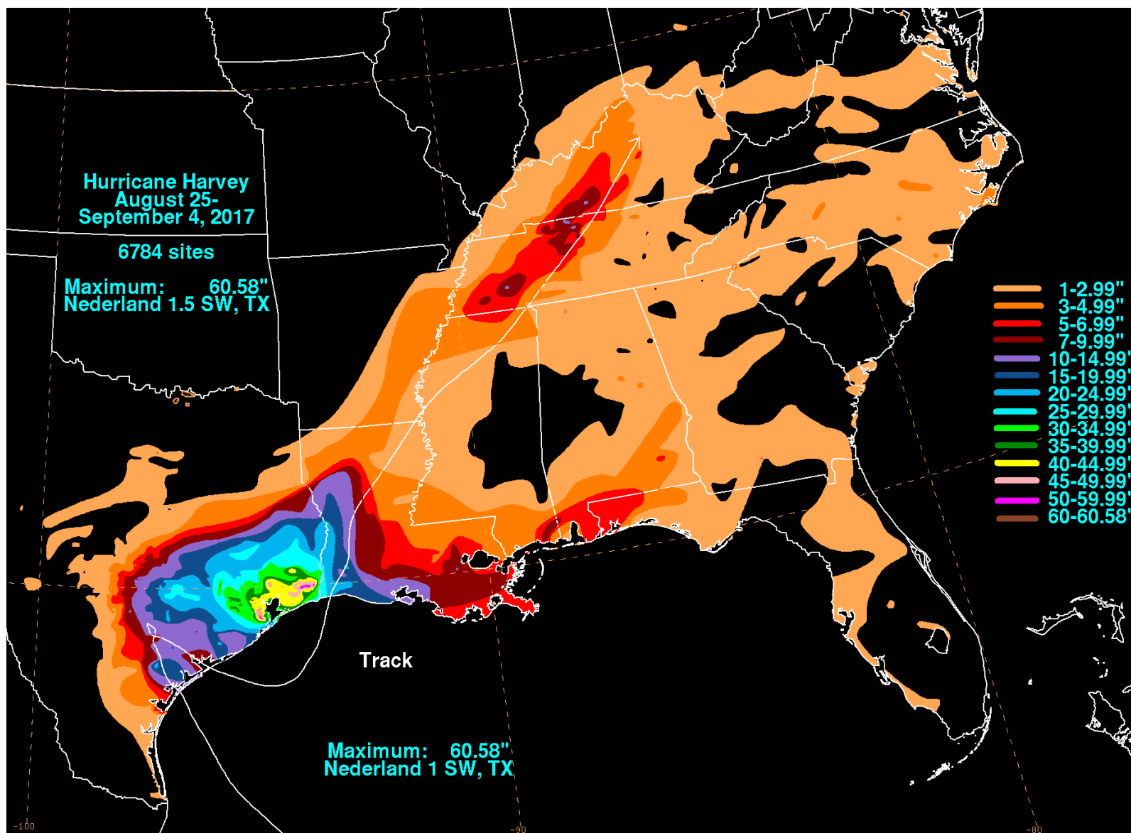
Figure 8. Observed rainfall totals (inches) in association with Harvey and its remnants. Figure courtesy David Roth (WPC).
