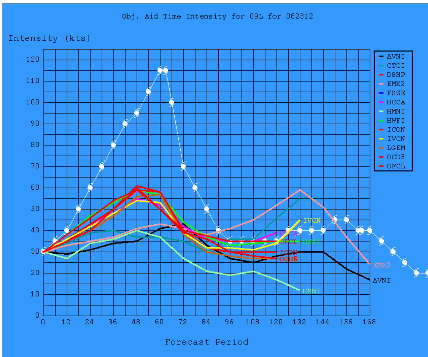
Figure 20. NHC intensity aids (knots, colored lines) for the 1200 UTC 23 August 2017 forecast cycle for Harvey (verifying points in white). Note the guidance was much too low for the intensity at landfall, which occurred near the 60-h point.
