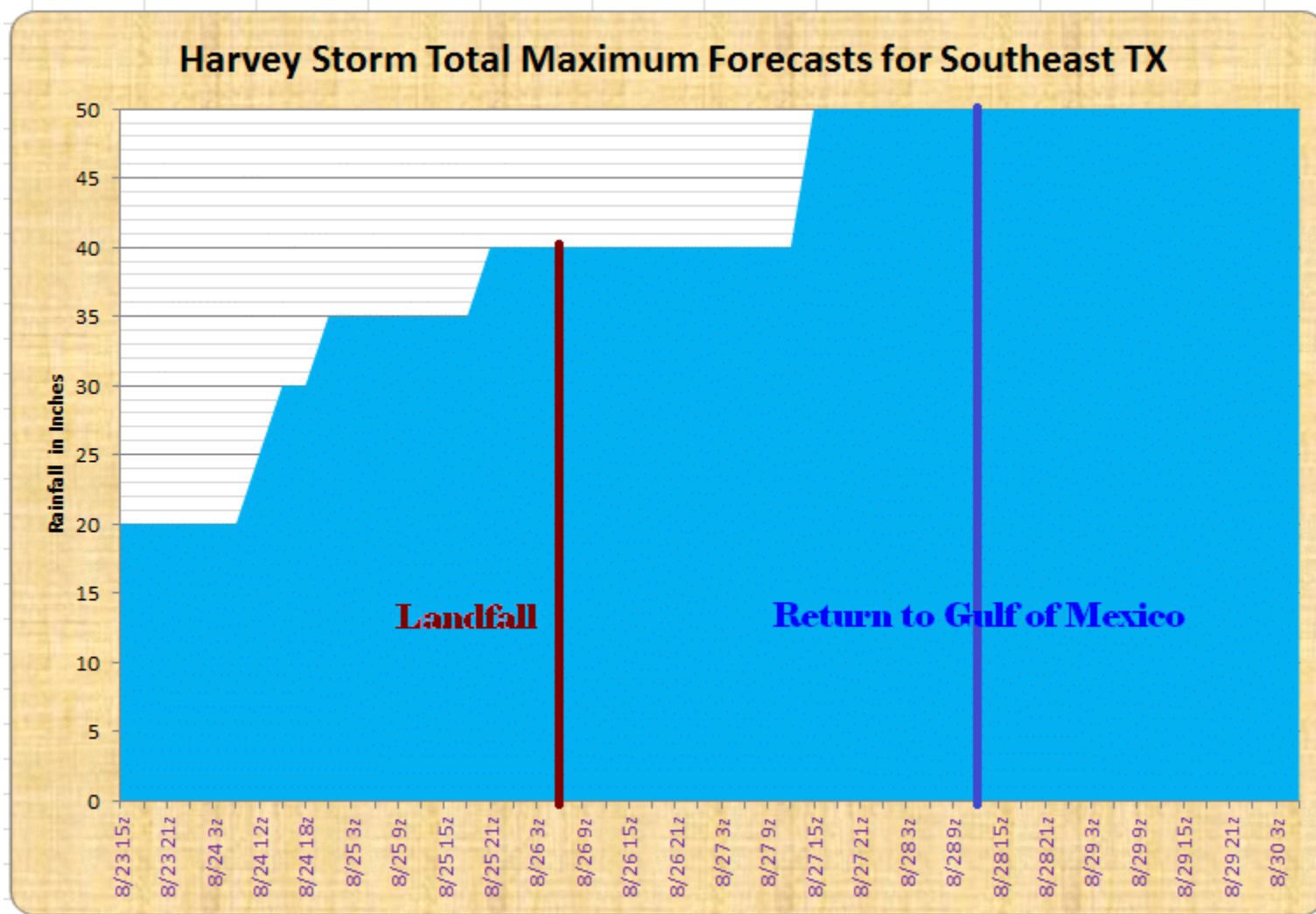
Figure 22. Time series of maximum rainfall forecasts for Harvey in southeastern Texas. Figure courtesy David Roth (WPC)
