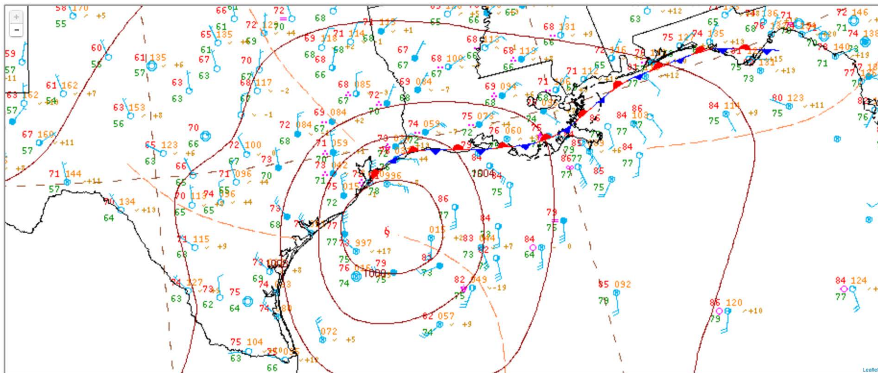
Figure 16. NCEP unified surface analysis at 1200 UTC 29 August 2017.
