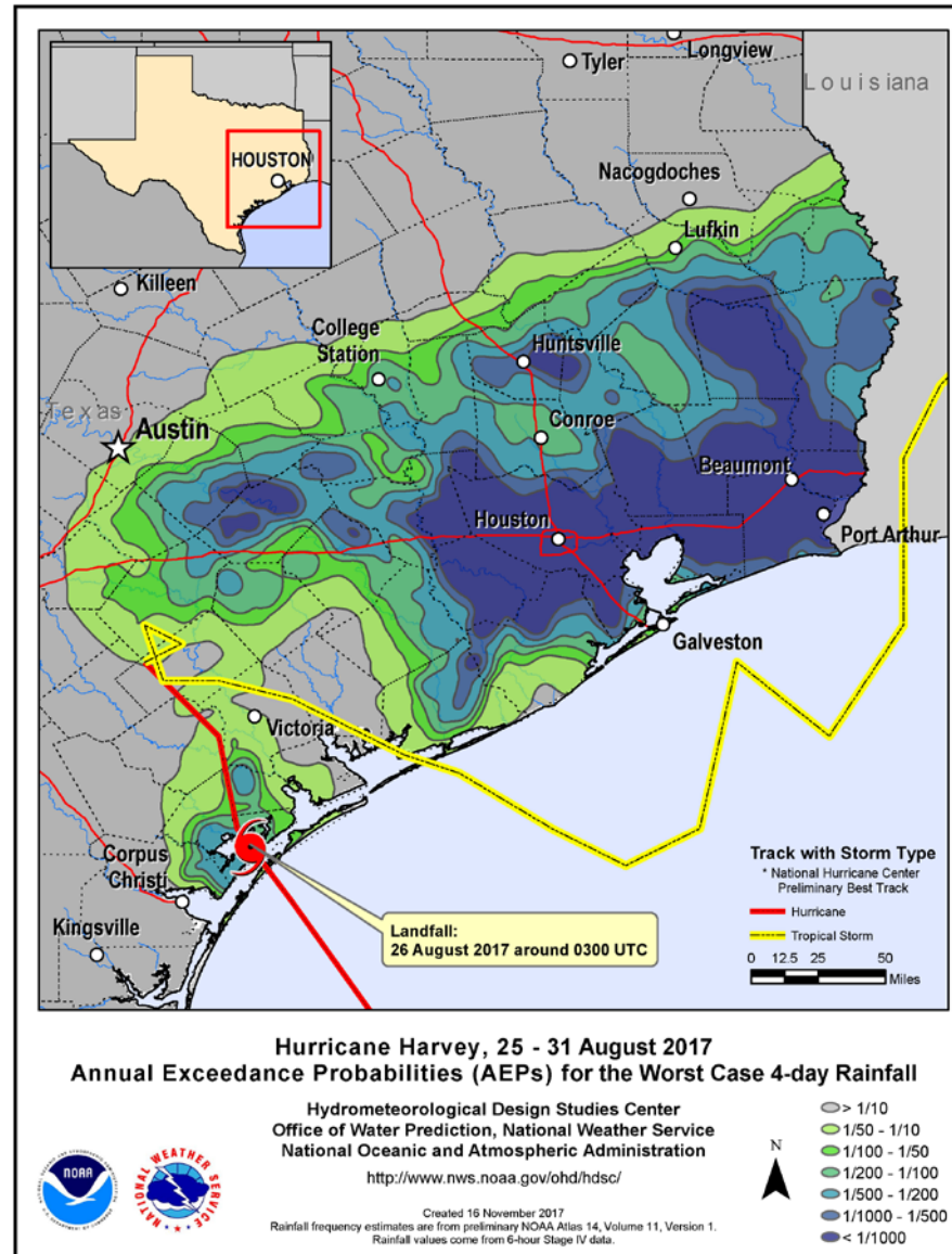
Figure 12. Annual 4-day rainfall exceedance probabilities for Harvey. Image courtesy NOAA Office of Water Prediction. Note that the track shown on the graphic was preliminary and does not reflect the final NHC best track.
