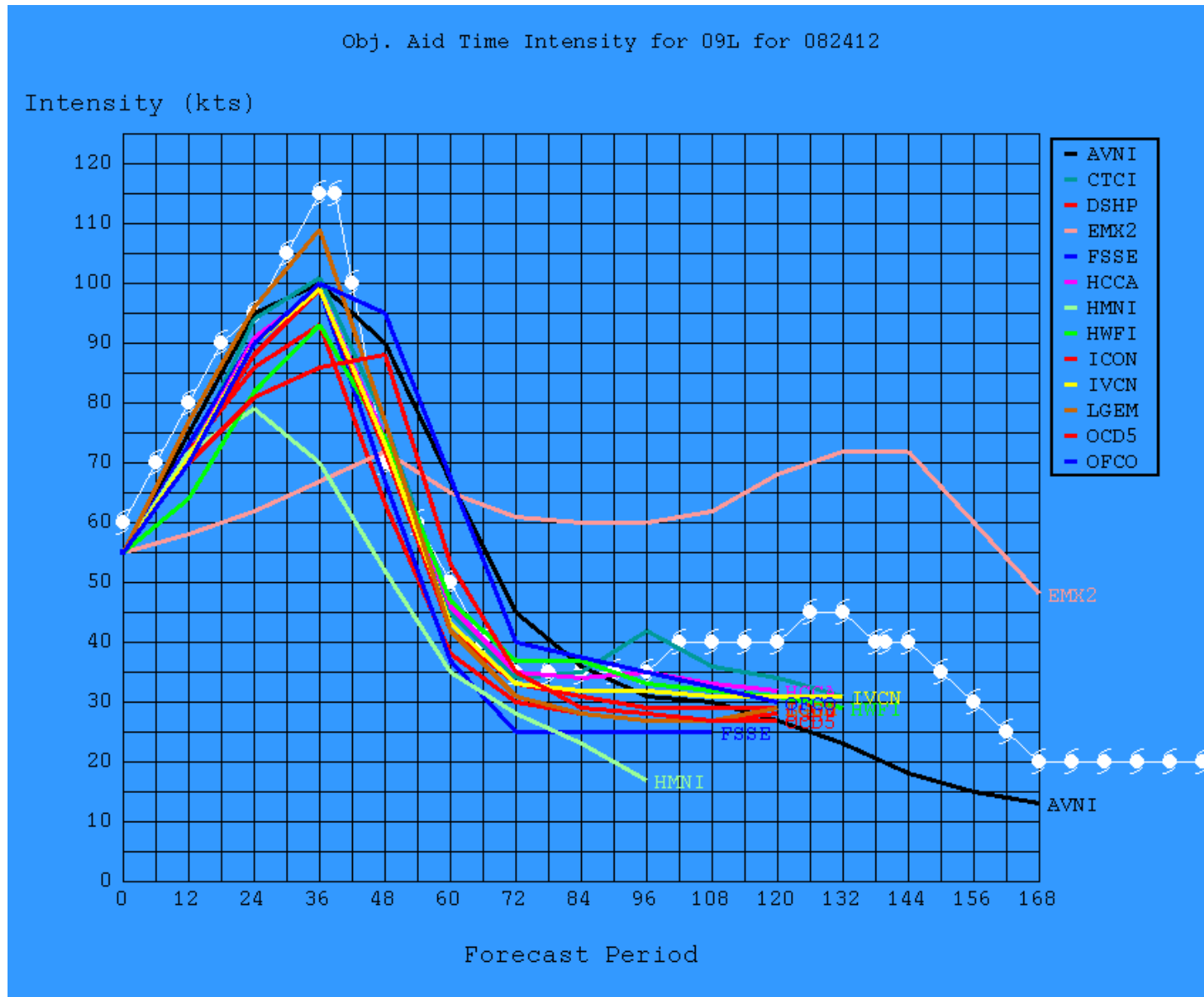
Figure 21. Same as Figure 20 but for 1200 UTC 24 August 2017. Note that much of the guidance showed rapid intensification before landfall, which occurred near the 36-h forecast point.
