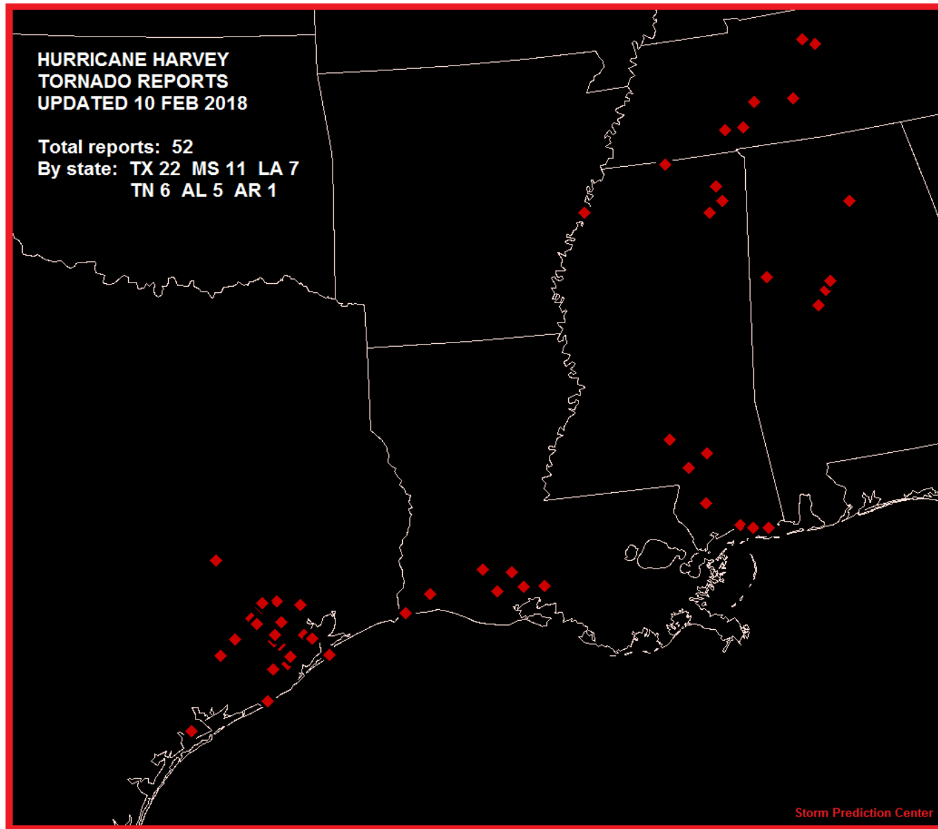
Figure 17. Tornado reports from Harvey. Figure courtesy Roger Edwards of the Storm Prediction Center.
