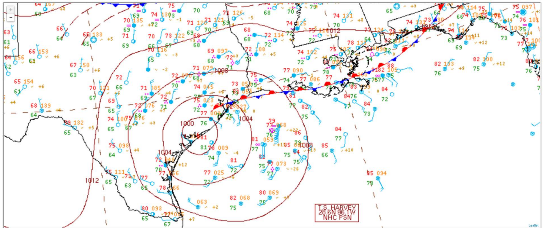
Figure 15. NCEP unified surface analysis at 1200 UTC 28 August 2017.
