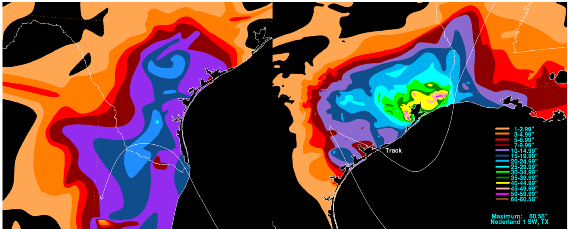
Figure 11b. As in Figure 11a except for Beulah (1967) rainfall (left).
