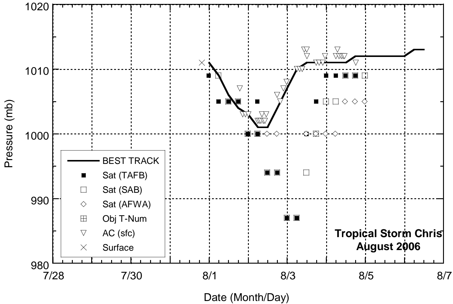
Figure 3. Selected pressure observations and best track minimum central pressure curve for Tropical Storm Chris, 1-4 August 2006.
