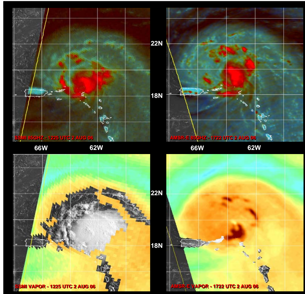
Figure 4. Microwave imagery from 1225 UTC 2 Aug 2006 SSMI (left) and 1722 UTC 2 AUG 2006 AMSR-E (right) overpasses showing the structure of Chris in 85GHZ data (top panels). The left panels show Chris near its peak intensity of 55 kt with a weak mid-level eye feature forming. The lower panels show mid-level dry air (blue and green shades) wrapping around the northern semicircle and intruding into the southwestern quadrant toward the center. (images from the U.S. Navy Research Laboratory, Monterey, CA).
