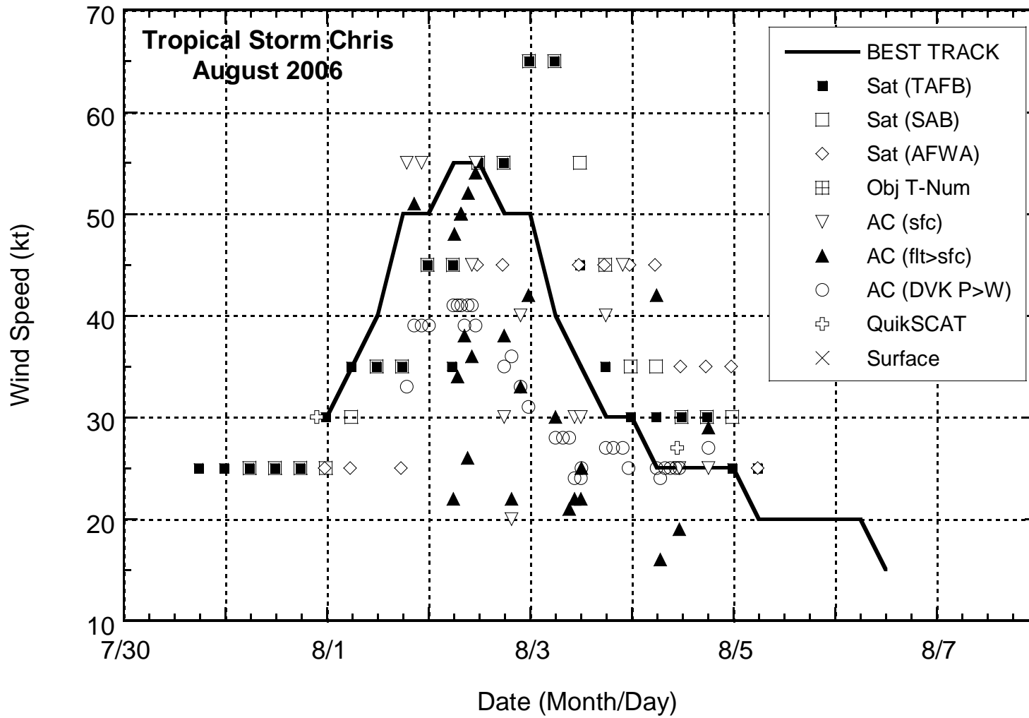
Figure 2. Selected wind observations and best track maximum sustained surface wind speed curve for Tropical Storm Chris, 1-4 August 2006.
