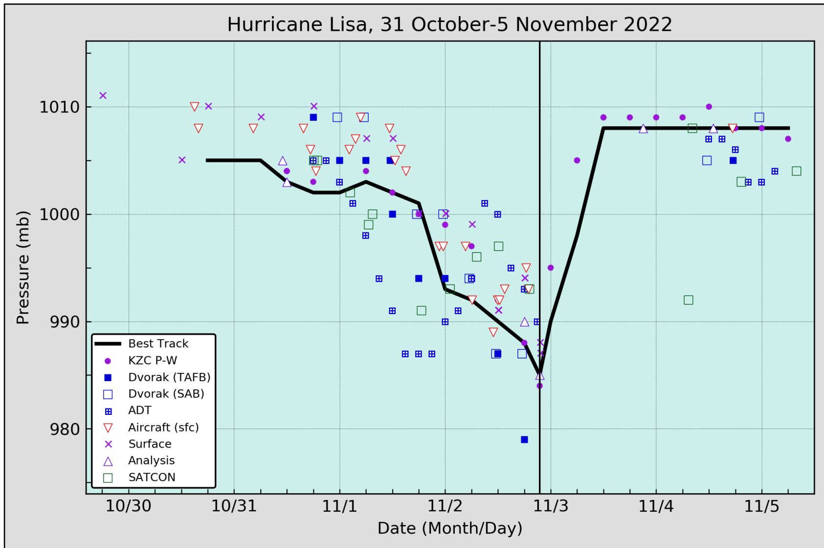
Figure 3. Selected pressure observations and best track minimum central pressure curve for Hurricane Lisa. Advanced Dvorak Technique estimates represent the Current Intensity at the nominal observation time. SATCON intensity estimates are from the Cooperative Institute for Meteorological Satellite Studies. KZC P-W refers to pressure estimates derived using the Knaff-Zehr-Courtney pressure-wind relationship. Dashed vertical lines correspond to 0000 UTC, and the solid line denotes landfall.
