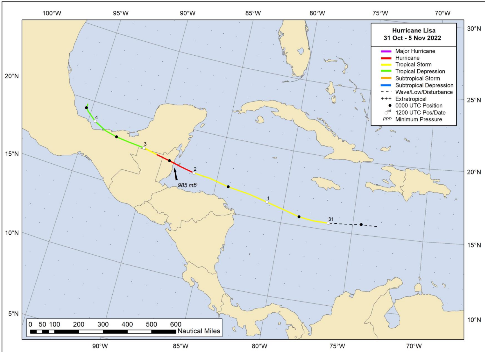
Figure 1. Best track positions for Hurricane Lisa, 31 October- 5 November 2022.
