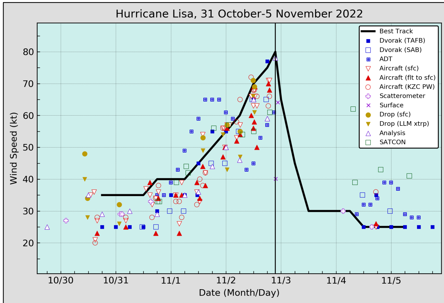
Figure 2. Selected wind observations and best track maximum sustained surface wind speed curve for Hurricane Lisa. Aircraft observations have been adjusted for elevation using 90%, 80%, 80%, and 75% adjustment factors for observations from 700 mb, 850 mb, 1500 ft, and 925 mb, respectively. Dropwindsonde observations include actual 10 m winds (sfc), as well as surface estimates derived from the mean wind over the lowest 150 m of the wind sounding (LLM). Advanced Dvorak Technique estimates represent the Current Intensity at the nominal observation time. SATCON intensity estimates are from the Cooperative Institute for Meteorological Satellite Studies. Dashed vertical lines correspond to 0000 UTC, and the solid line denotes landfall.
