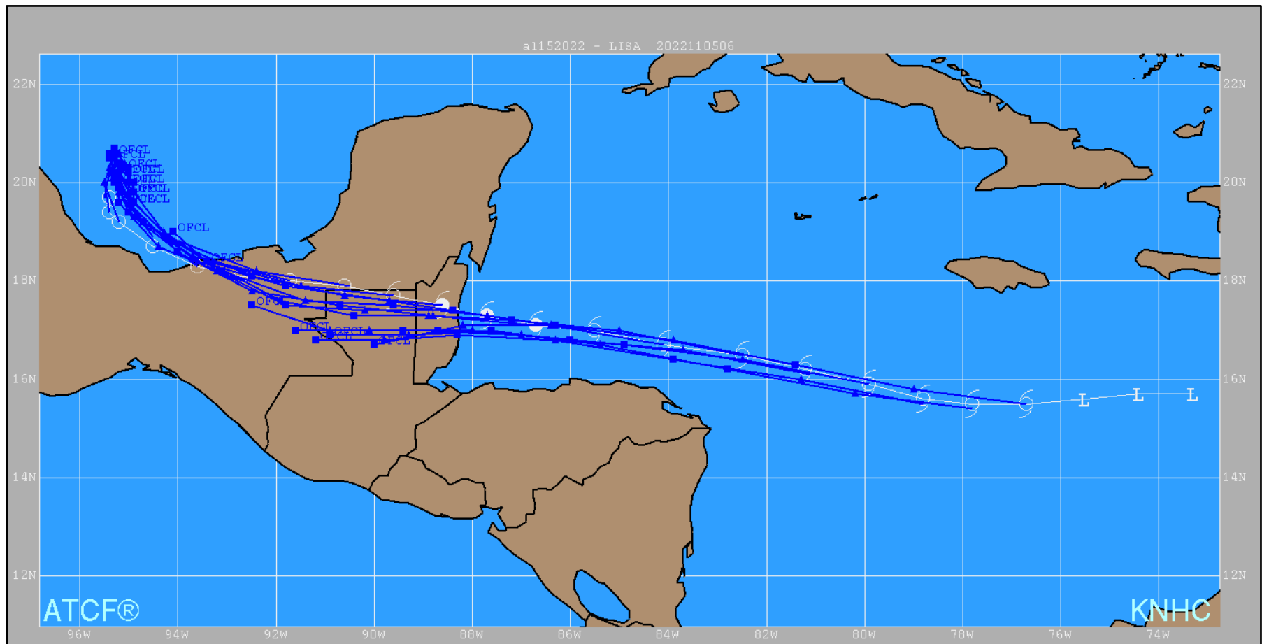
Figure 8. NHC 72-h track forecasts (blue lines) for Lisa after genesis (not including potential tropical cyclone forecasts). The verifying positions are shown in white.
