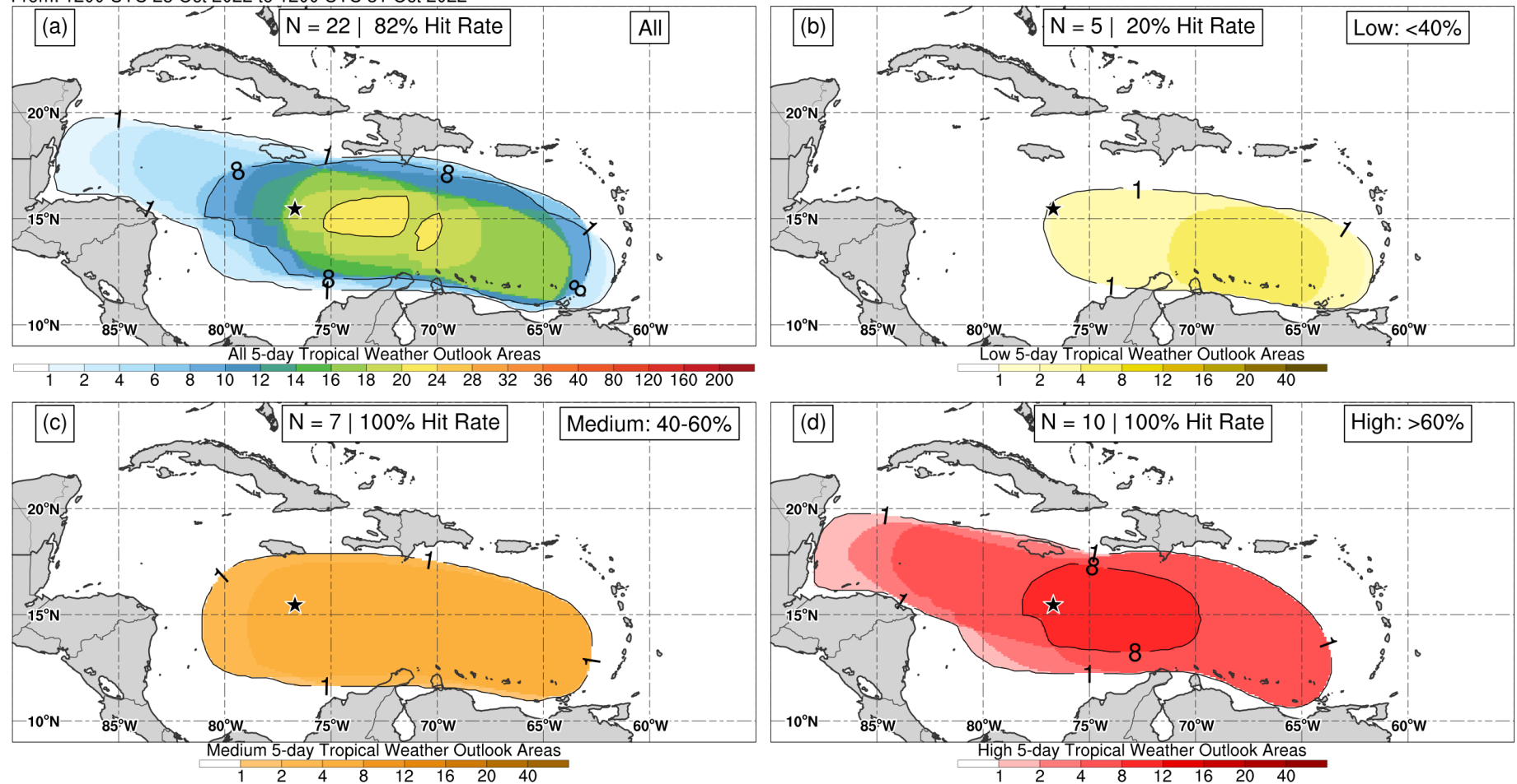
Figure 7. Composites of 5-day tropical cyclone genesis areas depicted in NHC’s Tropical Weather Outlooks prior to the formation of Hurricane Lisa for (a) all probabilistic genesis categories, (b) the low (<40%) category, (c) medium (40–60%) category, and (d) high (>60%) category. Lisa’s location of genesis is indicated by the black star.
